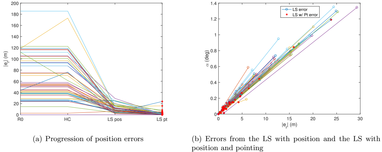
Figure 5.6: Evolution of position and pointing errors in the pre-processing algorithm when sampling from the Bennu lost-in-space orbit.
