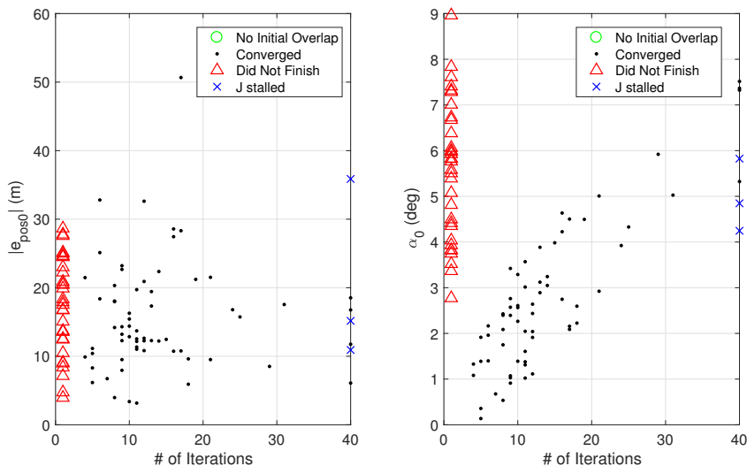
Figure 4.15: Magnitude of the initial position and pointing errors and their resulting LS MC outcomes for 1\sigma_r = 10\text{ m} , 1\sigma_{\theta_n} = 3^\circ .
